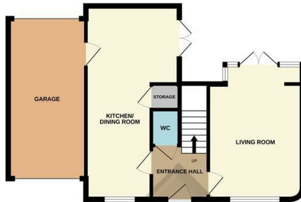
GROUND FLOOR 551 sq.ft. (51.2 sq.m.) approx.
